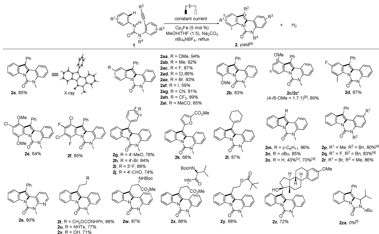
Scheme 2. Scope of indole synthesis. Reaction conditions: Reticulated vitreous carbon (RVC) anode, Pt cathode, constant current = 5 mA (ca. 0.05 mAcm -2 ), 1 (0.3 mmol), THF (7.5 mL), MeOH (1.5 mL), n Bu 4 NBF 4 (0.9 mmol), reflux, argon, 4 h (2.5 F). [a] Yield of isolated product.
