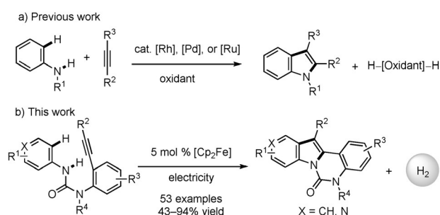
Scheme 1. (Aza)indole synthesis by C–H/N–H functionalization. Cp = cyclopentadiene.
