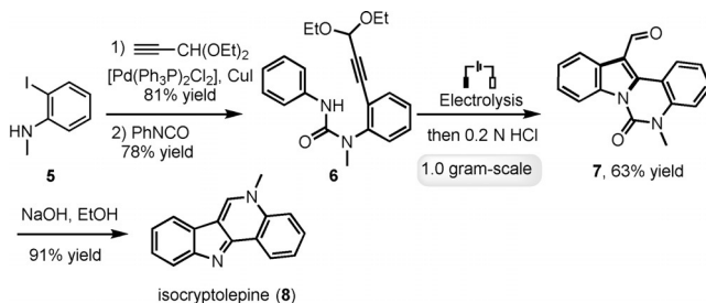
Scheme 4. Synthesis of the natural product isocryptolepine ( 8 ).
