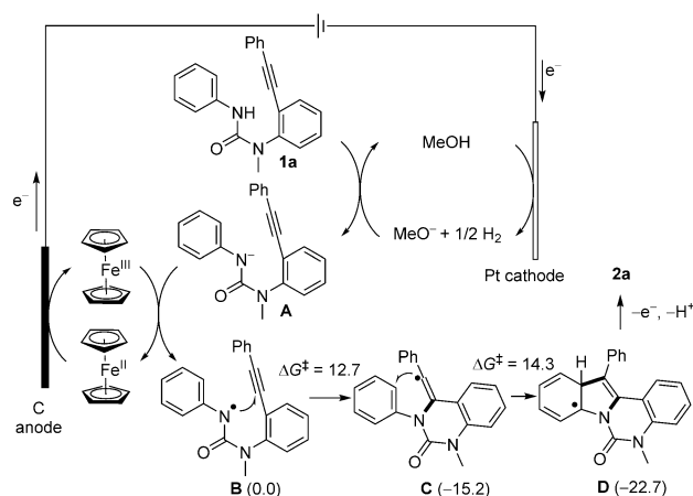
Scheme 5. Mechanistic proposal and computational studies. The values are DFT-derived energetics for the cyclization of the radical intermediate B . The energies (kcal mol −1 ), shown within parentheses, are those relative to B and were calculated at the level of B3LYP/6-31G*.
